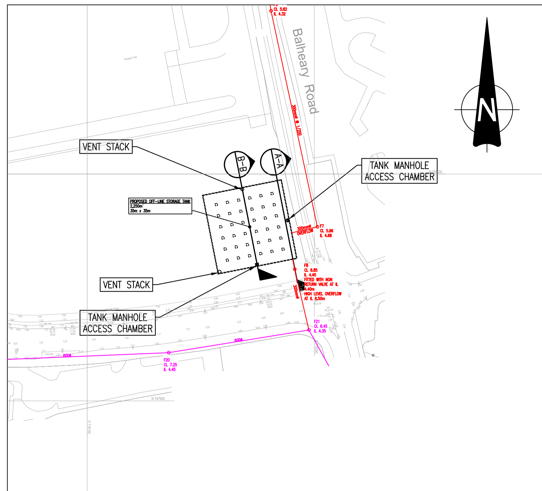
PLAN VIEW – DRAINAGE LAYOUT SCALE 1:1000 @A1
